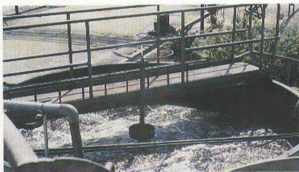
Effluent treatment: The Sequencing Batch Reactor developed by PORIM.
