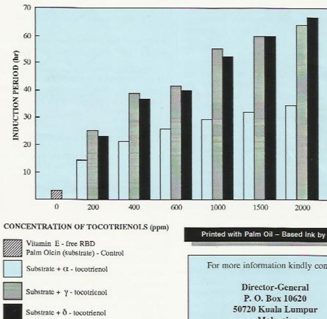
Figure 2. Antioxidant Activities of Tocotrienols in Vitamin E-free RBD Palm Olein.
