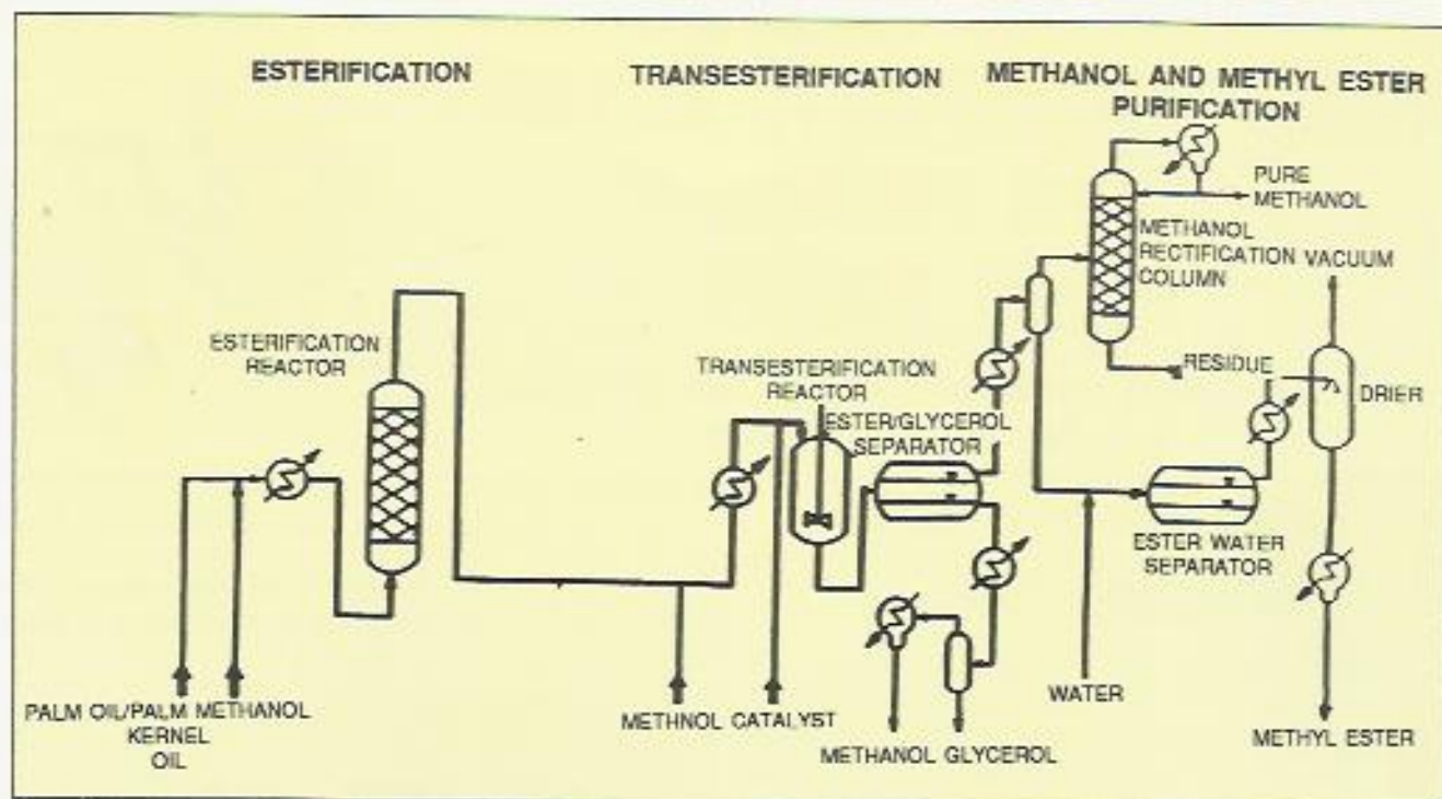
Figure 1. Methyl esters pilot plant
