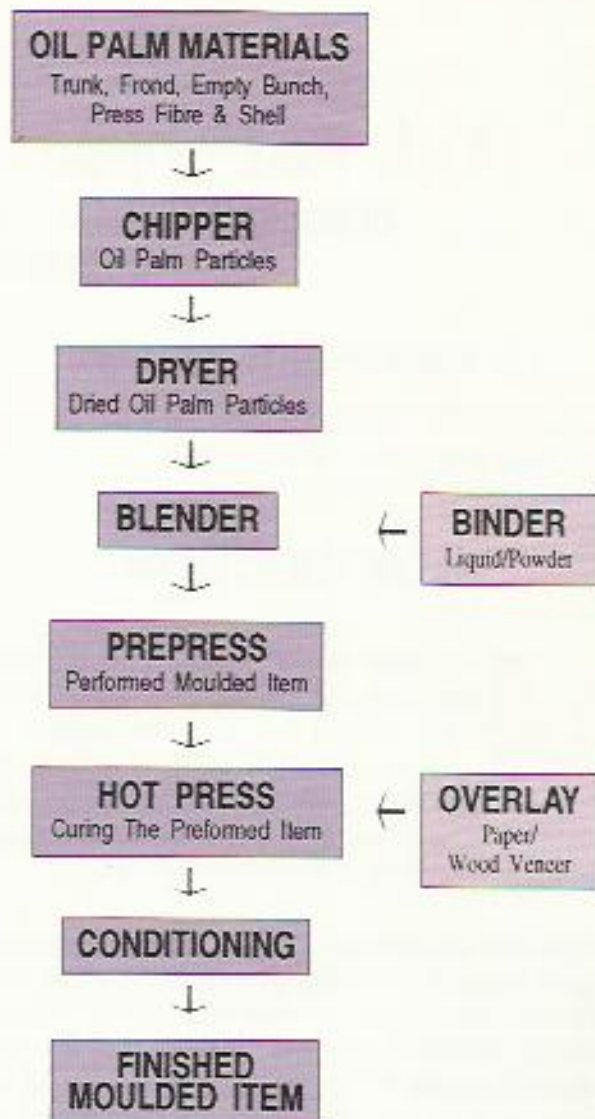
FIGURE 1. Process Flow Of Oil Palm Desk Tops And Chair Seats
